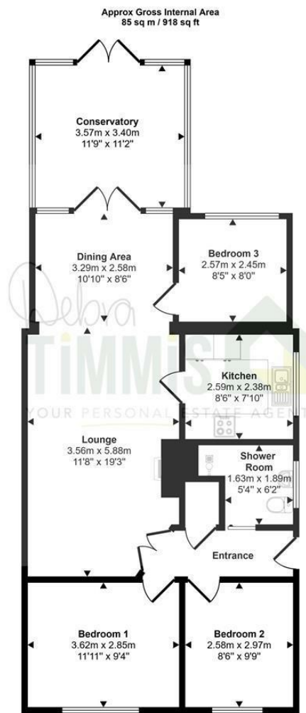
Floorplan
